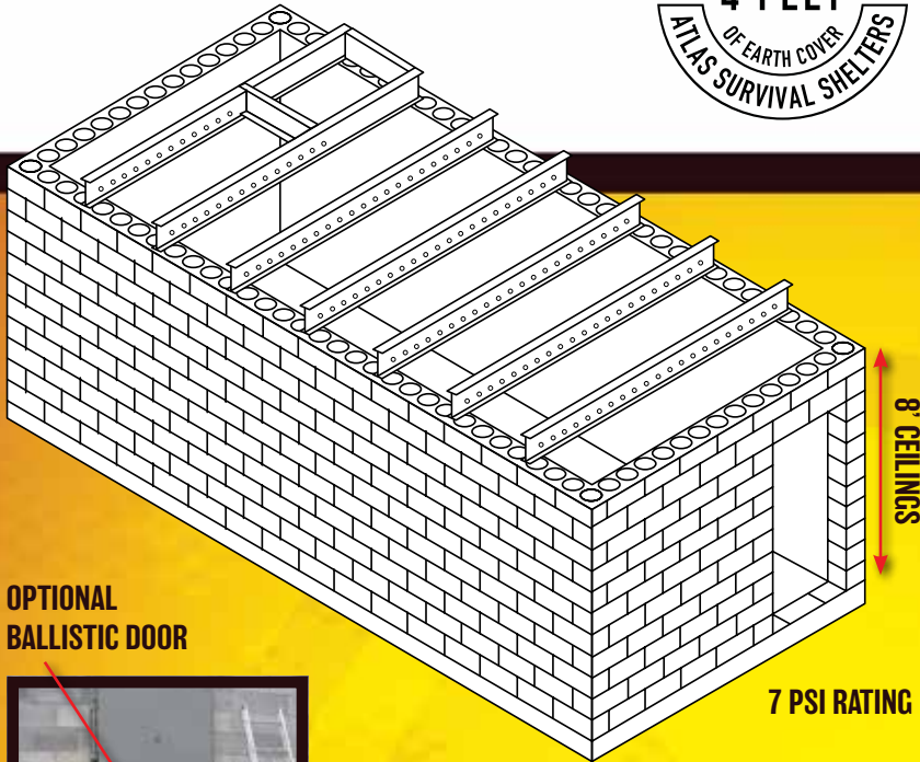
STANDARD ROOF ENTRY
