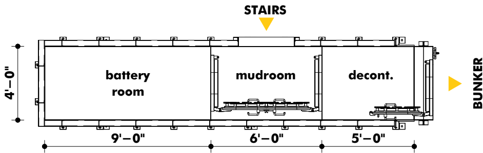
MUDROOM + DECONTAMINATION + BATTERY ROOM | 2
