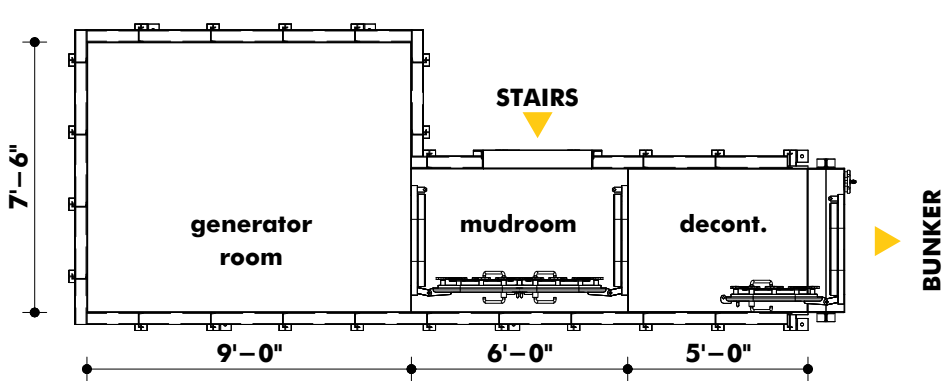
MUDROOM + DECONTAMINATION + GENERATOR | 3
